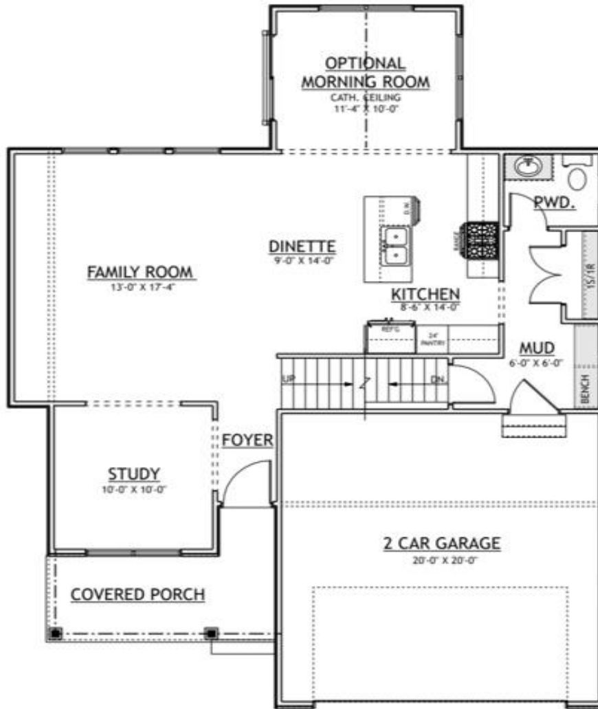
FIRST FLOOR PLAN 943 SQ. FT.
